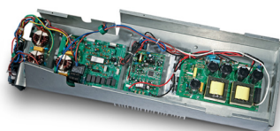
Inverter Controller for Large System
